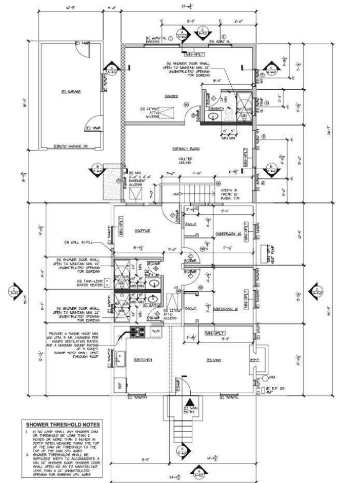
2 PROPOSED MAIN HOUSE FLOOR PLAN SCALE = 1/4" = 1'-0"
